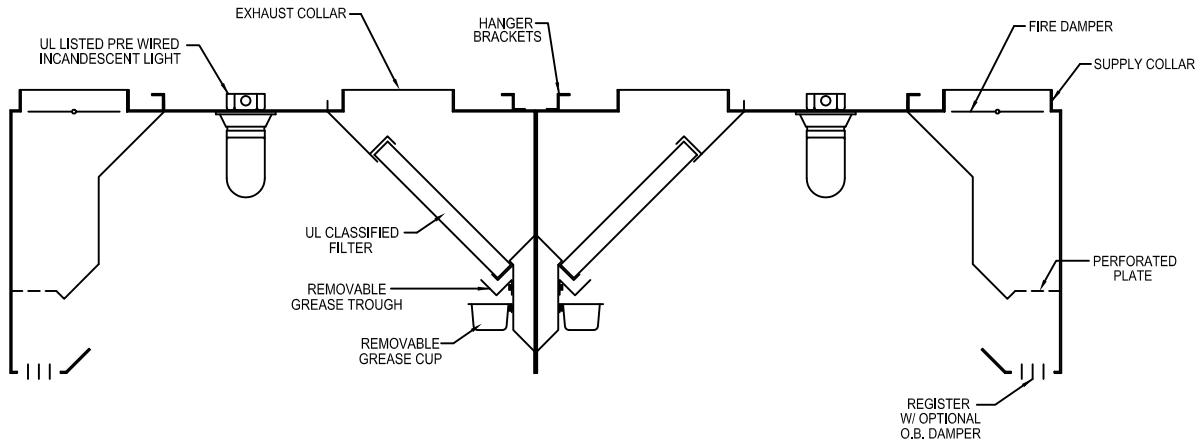
SECTION VIEW
