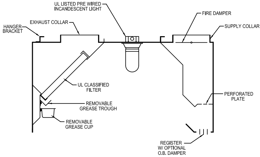
SECTION VIEW
