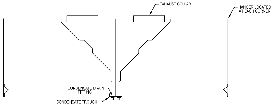
SECTION VIEW
