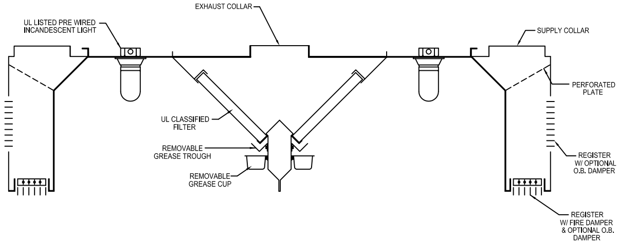
SECTION VIEW
