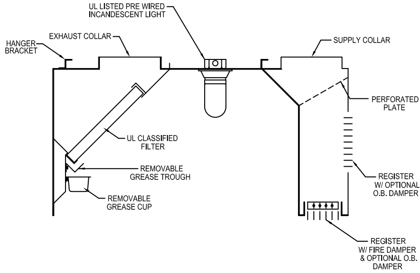
SECTION VIEW
