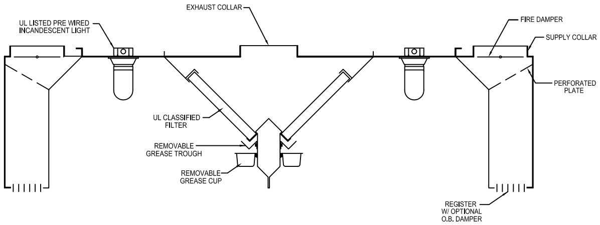
SECTION VIEW
